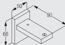
0989 Blok Bracket
